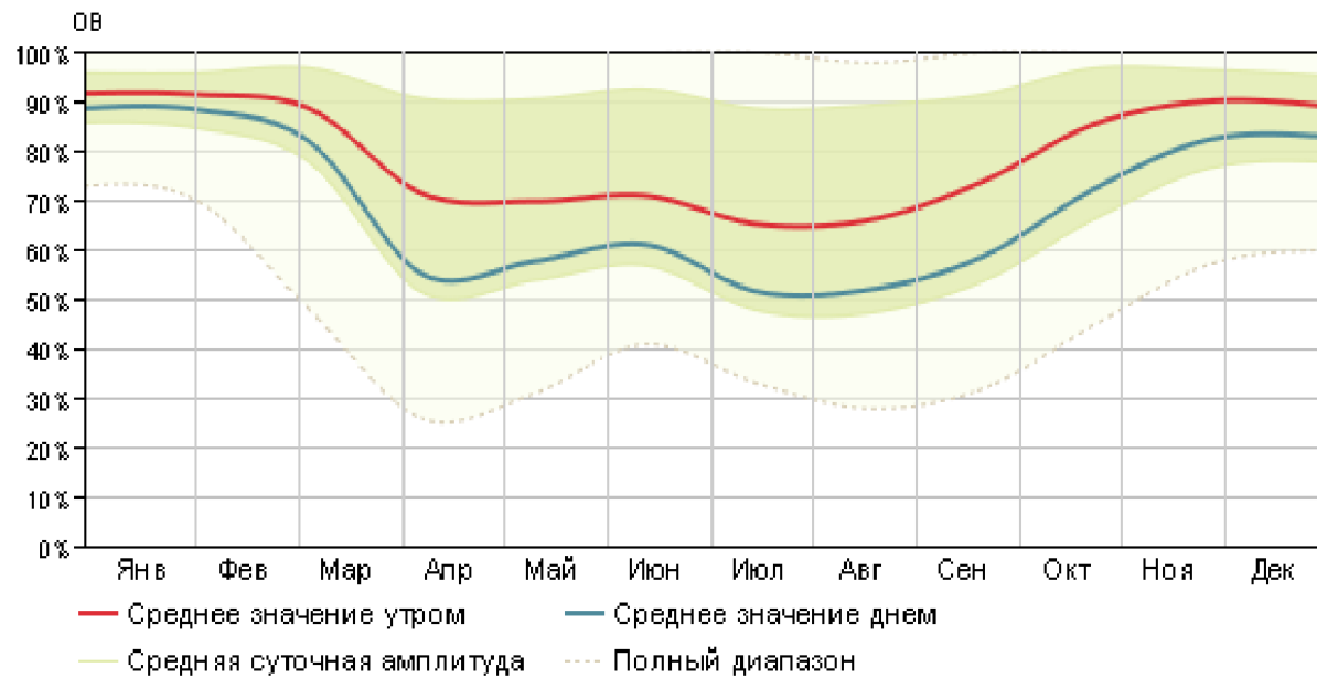
Fig. 30. Annual distribution of relative humidity
