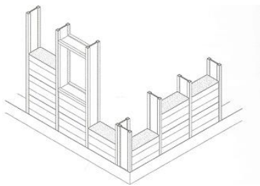
Fig. 5. I-section rack
