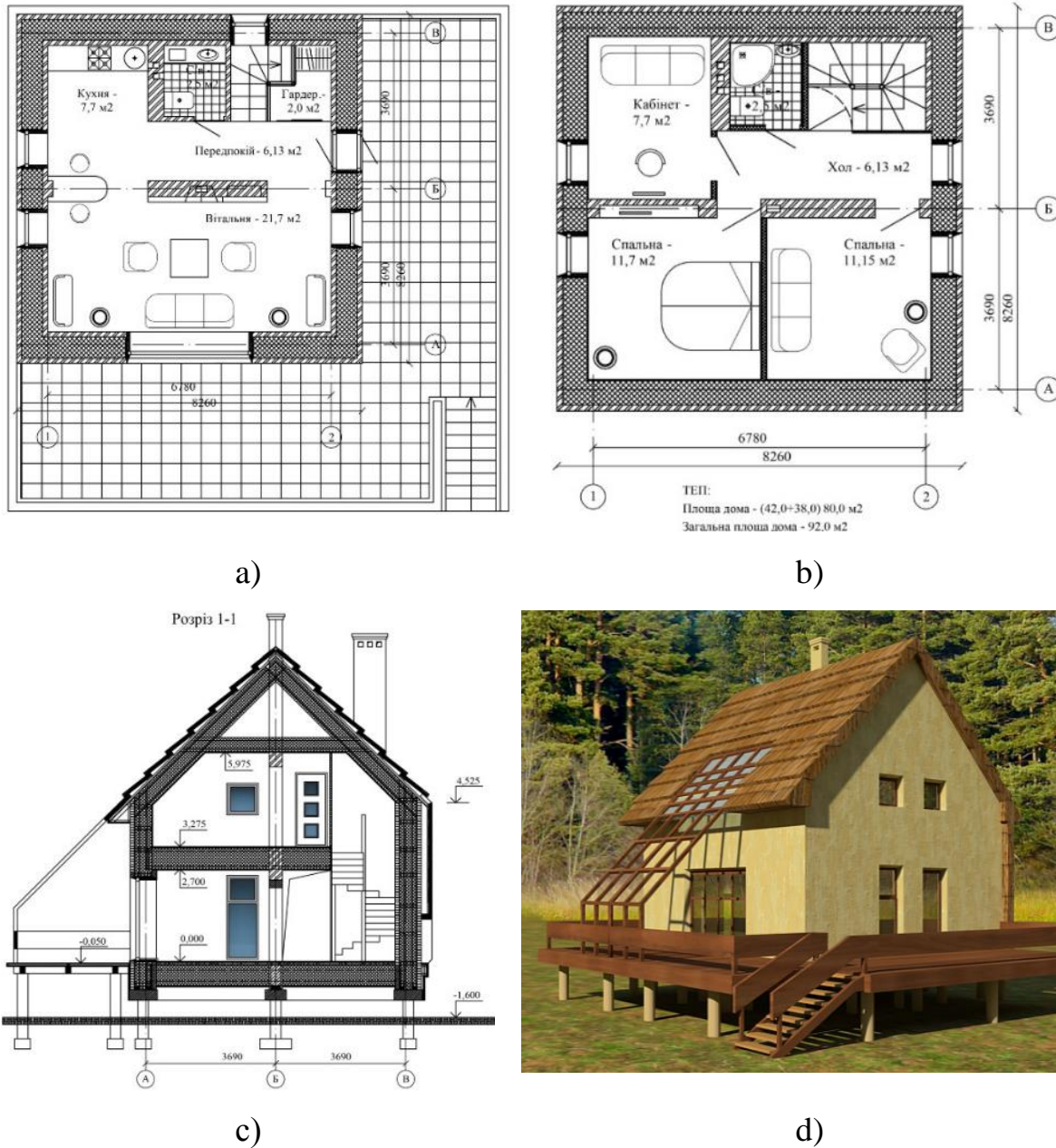
Fig. 22. Triple Net Zero Building: a) first floor layout; b) attic floor layout; c) cross-section; d) 3d visualization
